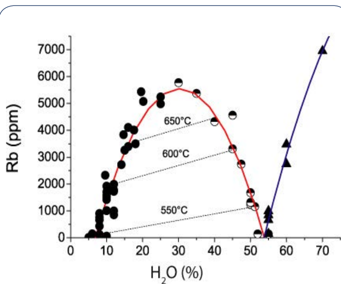
Figure 2: Plot of the Rb concentration in melt and fluid inclusions versus the water content. Black points represent the so-called A-type melt inclusions, and half-filled points represent the water-rich B-type melt inclusions, and the black triangles stand for fluid inclusions. The isotherms are drawn in for both melt inclusion types.
