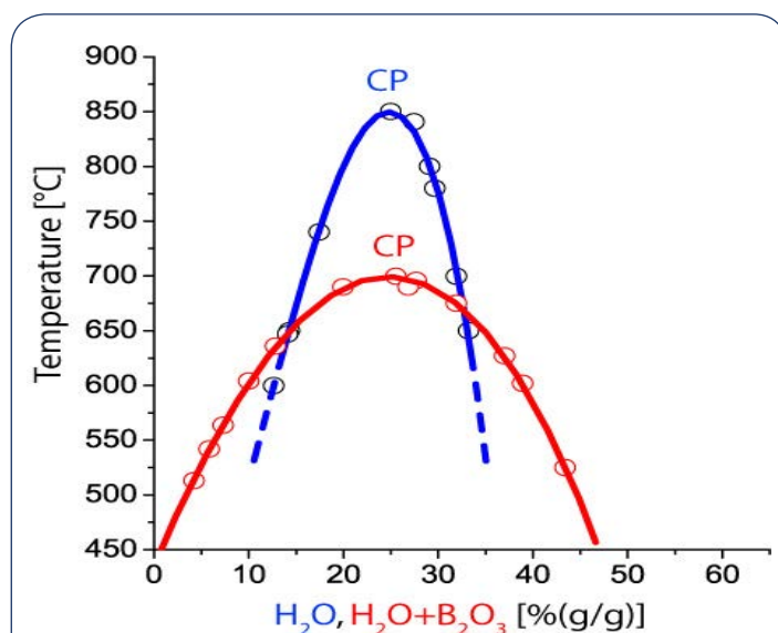
Figure 1: Pseudobinary solvus curves of evolved granites (blue) and pegmatites (red) for the Ehrenfriedersdorf tin deposit. CP – critical point. The critical point for the F-rich granites is 850°C and 25% H 2 O, and for the pegmatites, the CP is 712°C and 27.7% (H 2 O + B 2 O 3 ).
